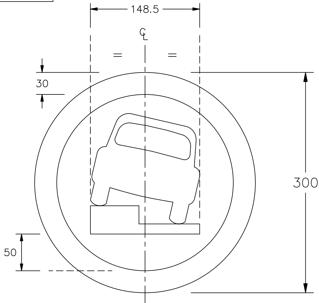
Symbol dimensions shown on dwg P 667 1sw = 11mm
