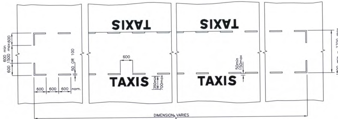
TAXI RANK IN CENTRE OF THE CARRIAGEWAY (RED OR YELLOW) REF : E2
