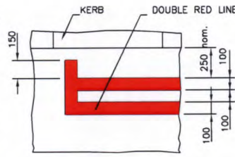
DOUBLE RED LINE - TERMINATION REF : B1
