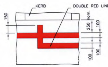
SINGLE/DOUBLE RED LINE - TRANSITION
