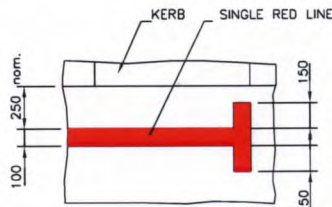
SINGLE RED LINE - TERMINATION REF : A1
