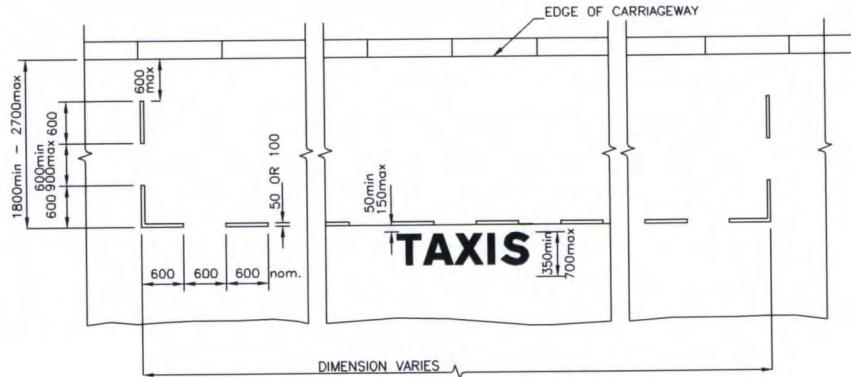
TAXI RANK ADJACENT TO KERB (RED OR YELLOW) REF : E1
