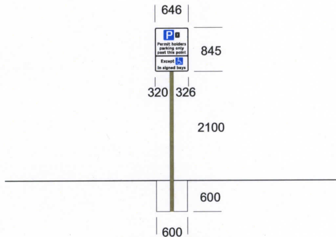
Foundation length: 1000 Not to scale
