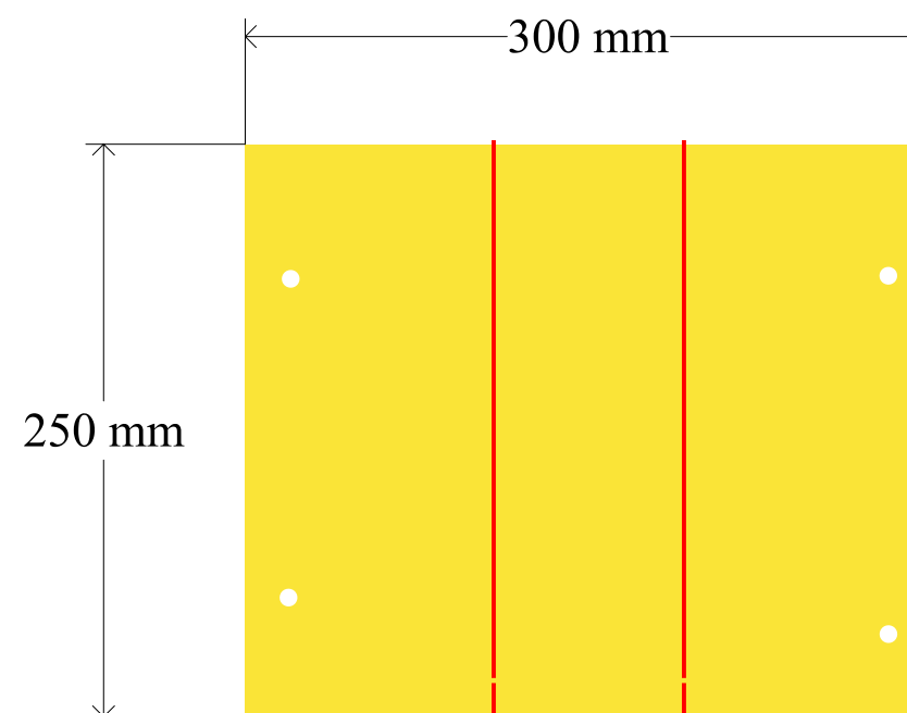
Back panel
