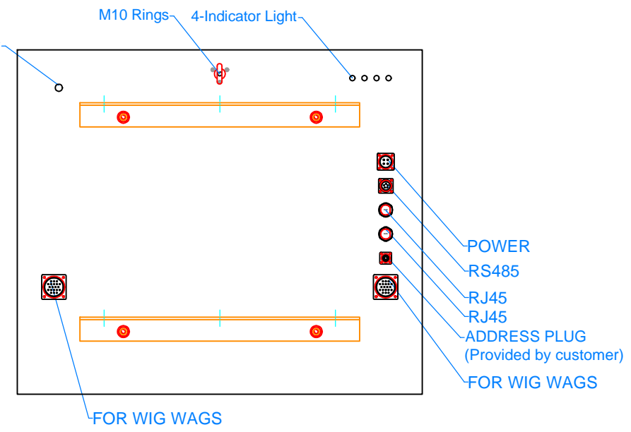
REAR VIEW
