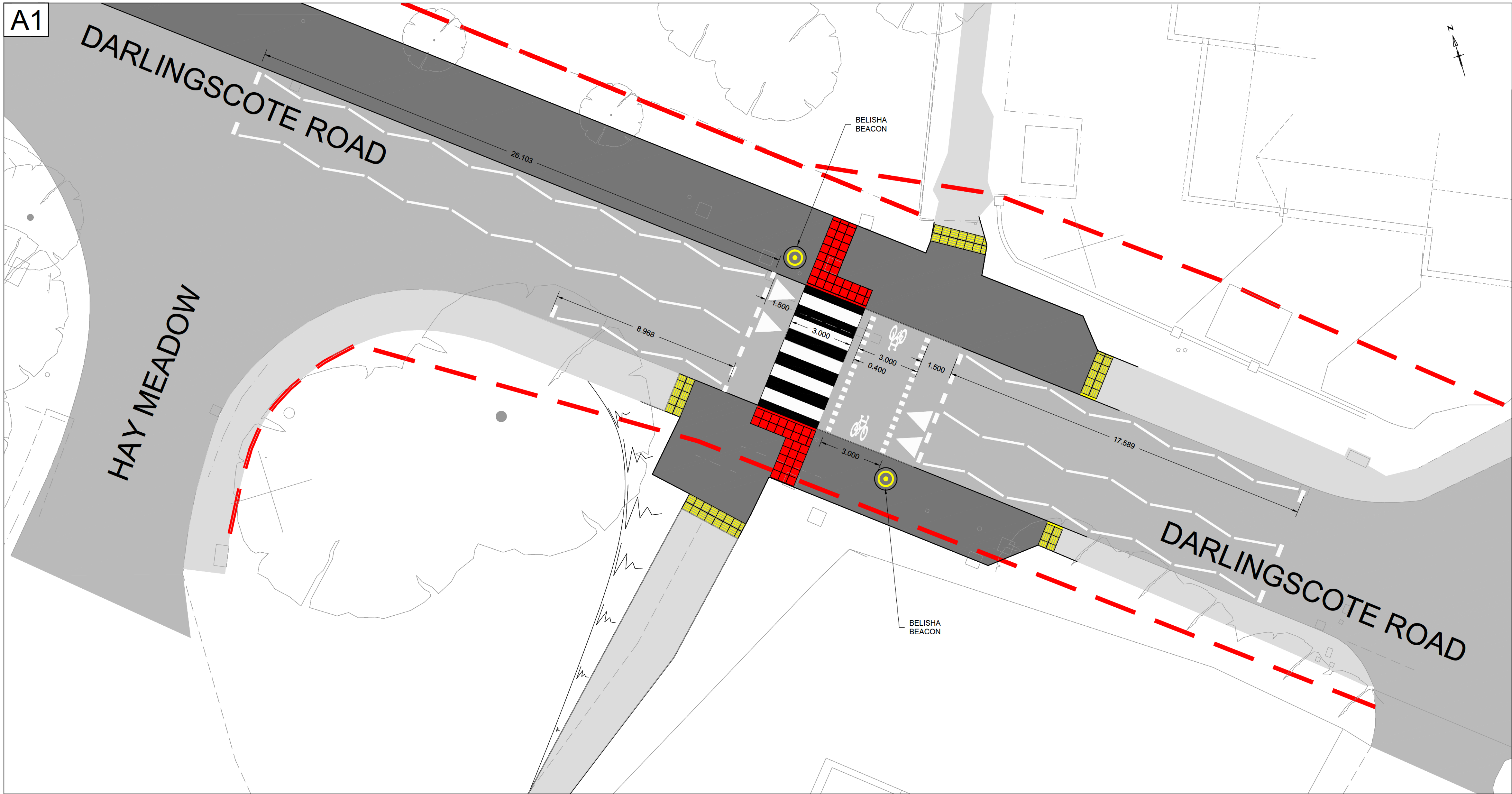
INSET A PARALLEL CROSSING ON ROAD HUMP DARLINGSCOTE ROAD SCALE 1 : 100
