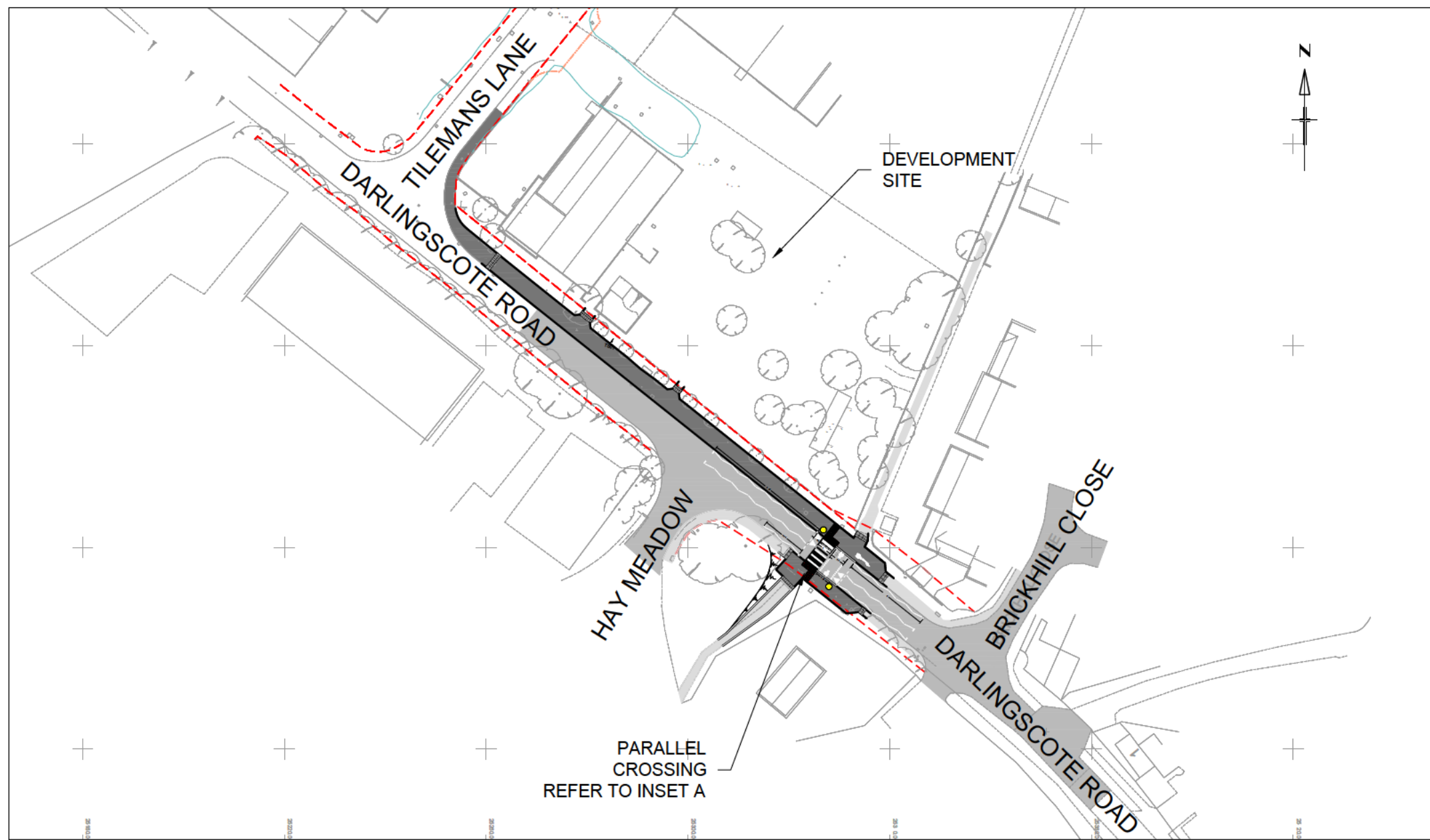
LOCATION PLAN SCALE 1 : 1,000
